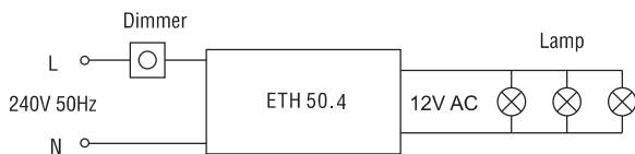
Wiring Diagram
