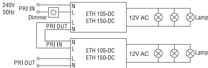
Wiring Diagram
